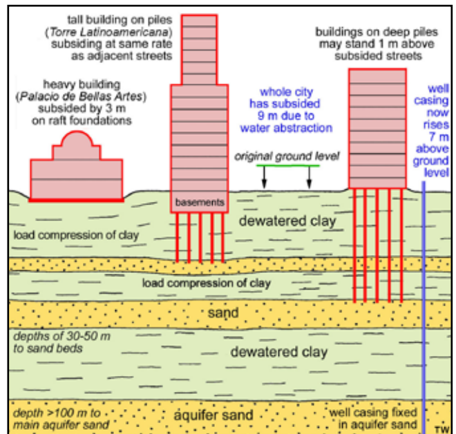
Schematic profile of the ground beneath Mexico City.
